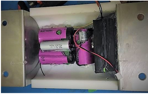
Figure 11: Commercial GPS tracking unit extended with the gunshot detection subsystem before being filled with resin. The protective black box contains the acoustic sensor board and the delay line. One of the batteries (purple cylinders) is reserved for the gunshot detector and the remaining ones for the tracking unit (located underneath). Additional supercapacitors (grey cylinders) are included to help with the current spikes of the GPS and the SD card.
