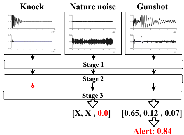
Figure 10: The structure and the behavior of the detector with three example recordings propagating through the stages. In these recordings on the top, the upper signals correspond to the contact microphone, the lower ones to the electret microphone.
