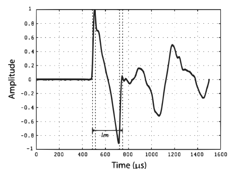
Figure 1: Shockwave of an M16 projectile
