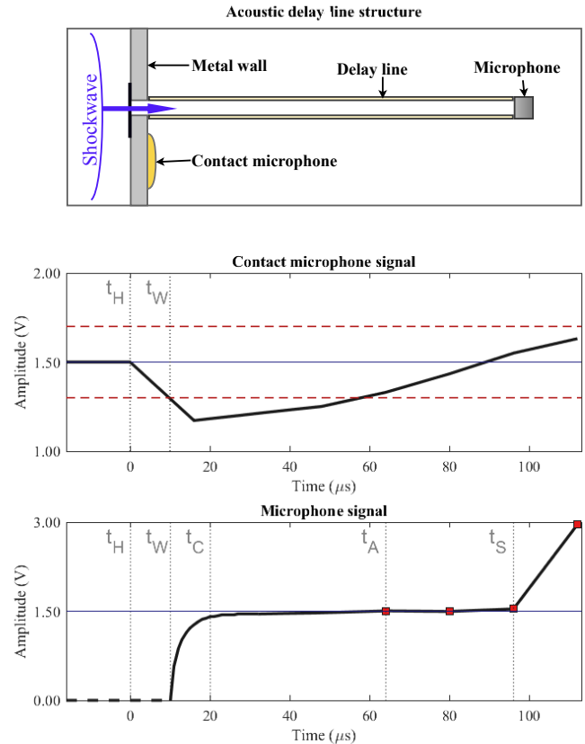
Figure 4: Details of the wake-up mechanism. In the top row the structure of the delay line and the propagation of a shockwave from left to right are shown. Below that, the microphones' signals synchronized to the shockwave's progress are plotted. Different time points of the event are marked: t_H - the shockwave hits the wall; t_W - wake-up signals are generated by the contact microphone; t_C - CPU and microphone switch to active mode; t_A - the first ADC sample is collected; t_S - the shockwave reaches the microphone.
